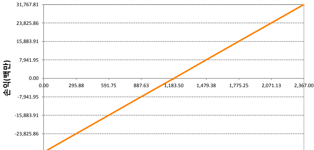
LBMA20200916-LBMA골드ICBC20200916
